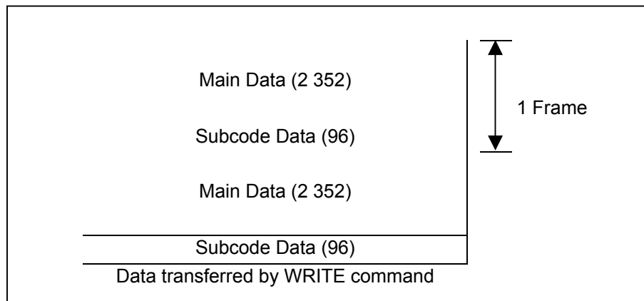
Figure 128 — Location of Sub-channel Data
