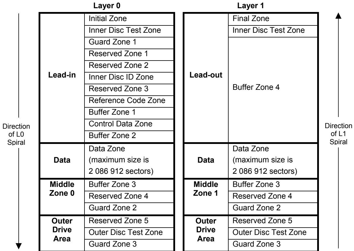
Figure 58 — Logical Layout of a DVD+RW DL Disc
