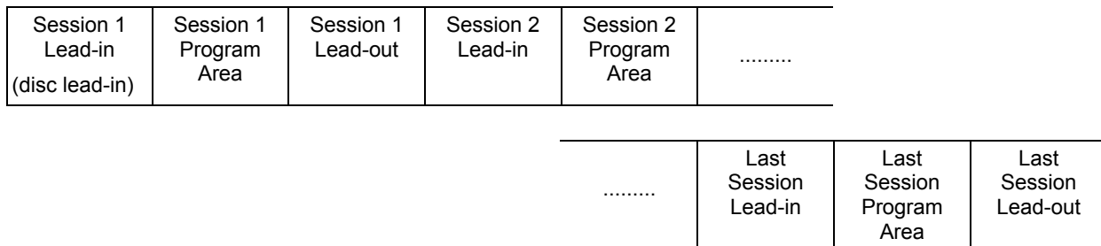
Figure 11 — Multi-Session Recorded Disc
