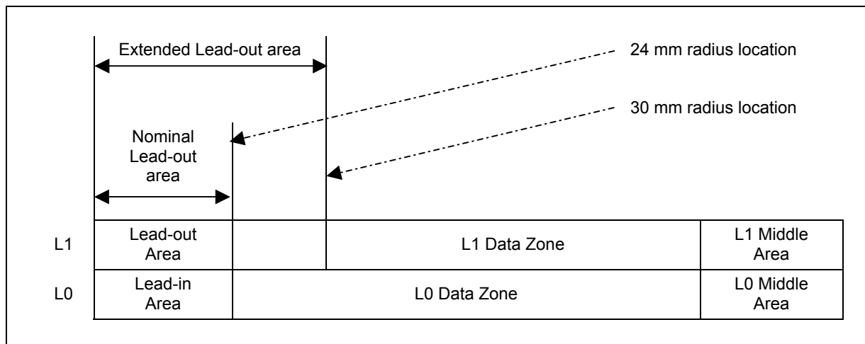
Figure 55 — Finalization Areas on DVD+R DL
