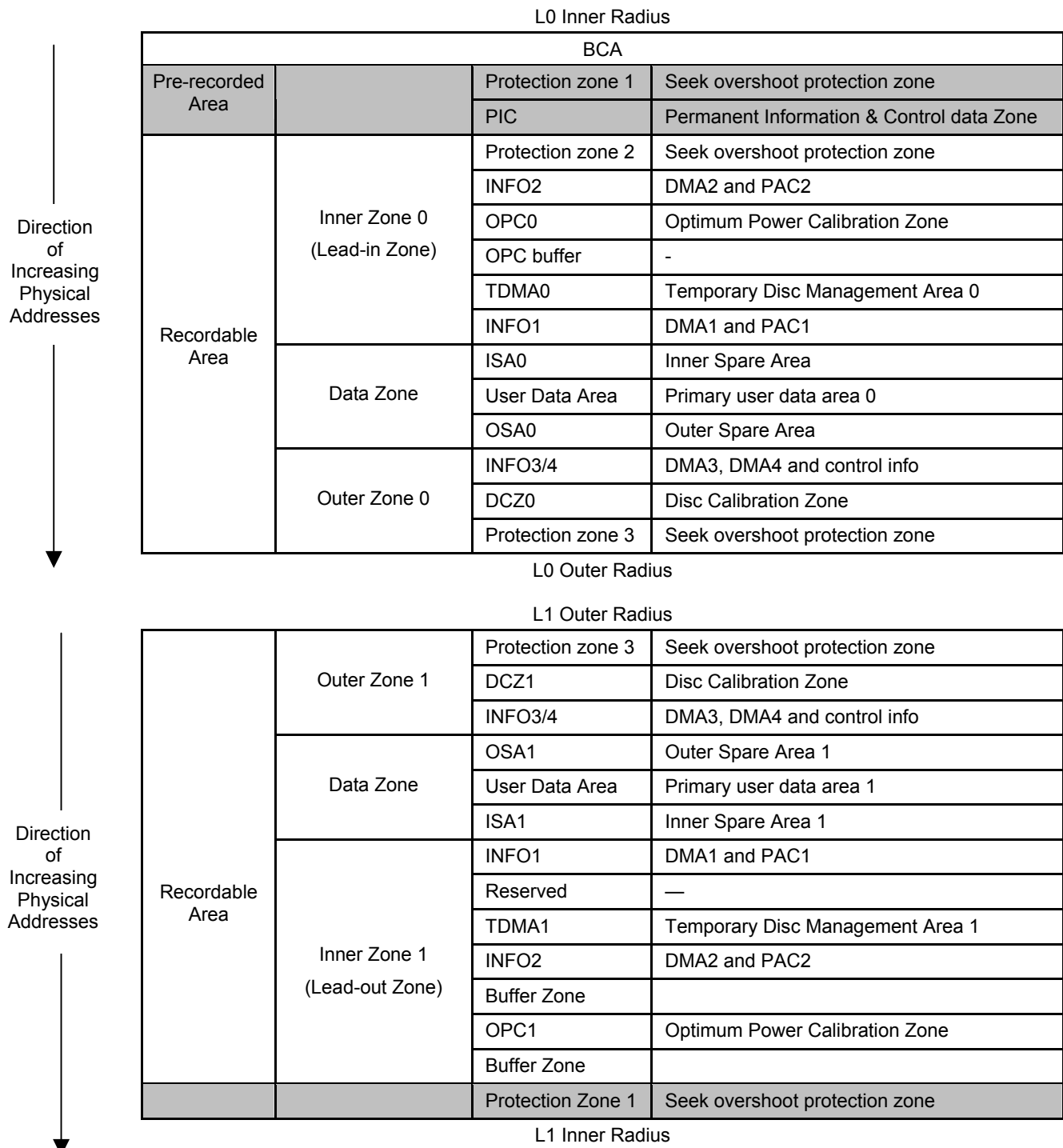
Figure 82 — BD-R Information Zones
