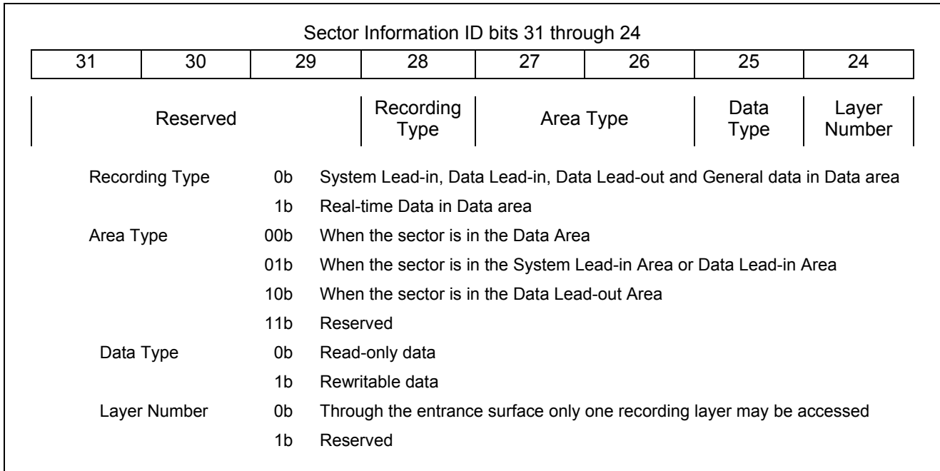
Figure 75 — HD DVD-RAM ID field Sector Information details
