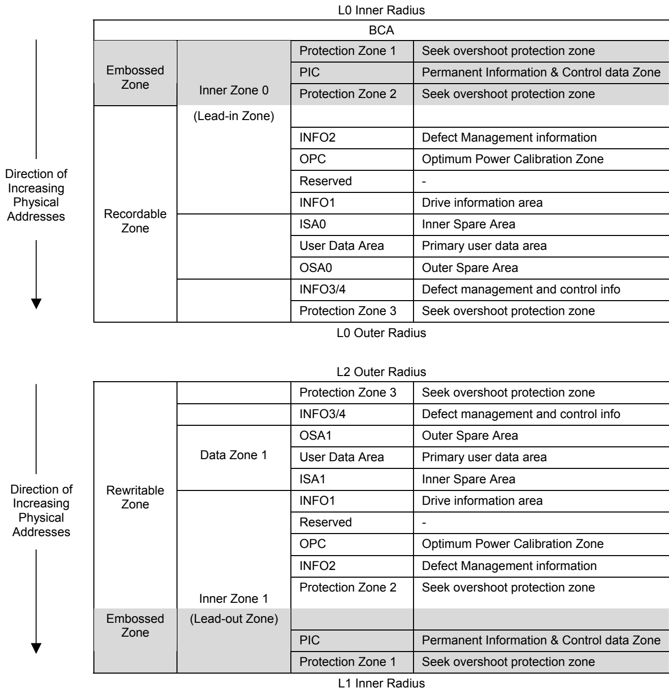
Figure 105 — BD-RE Information Zone
