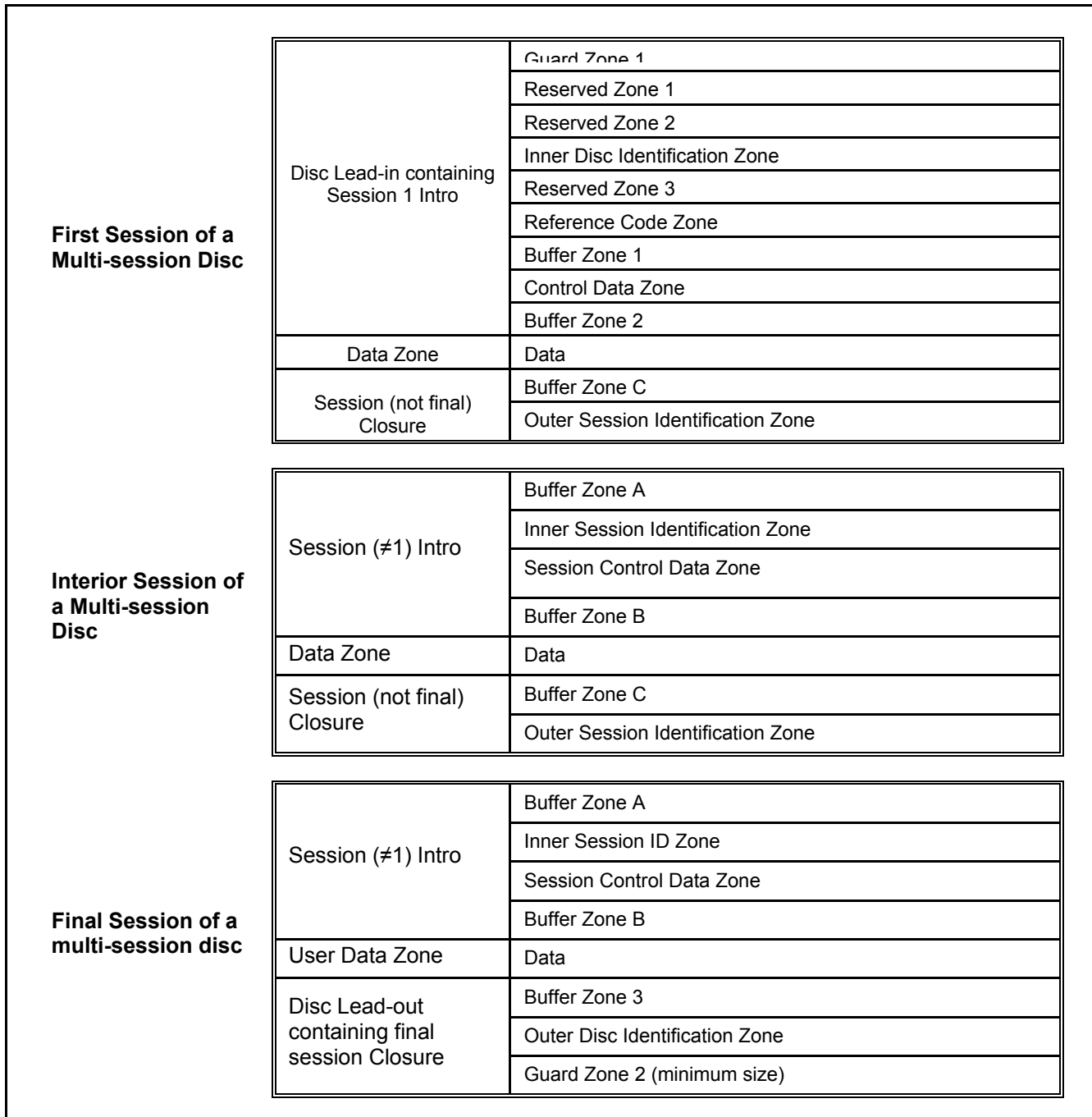
Figure 47 — Zones of a Session
