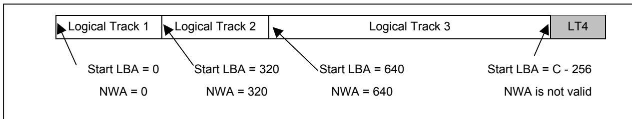
Figure 98 — Status after Splitting Logical Track 2
