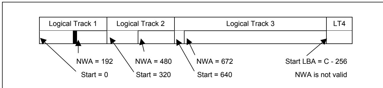
Figure 100 — Status after LOW to LBA 256
