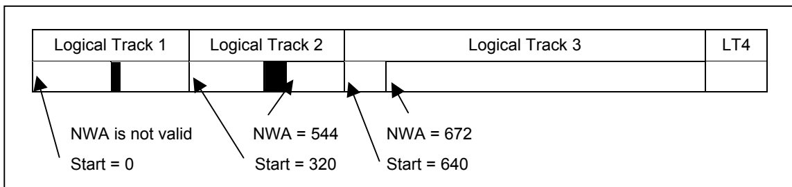
Figure 102 — Status after LOW of LBA 256
