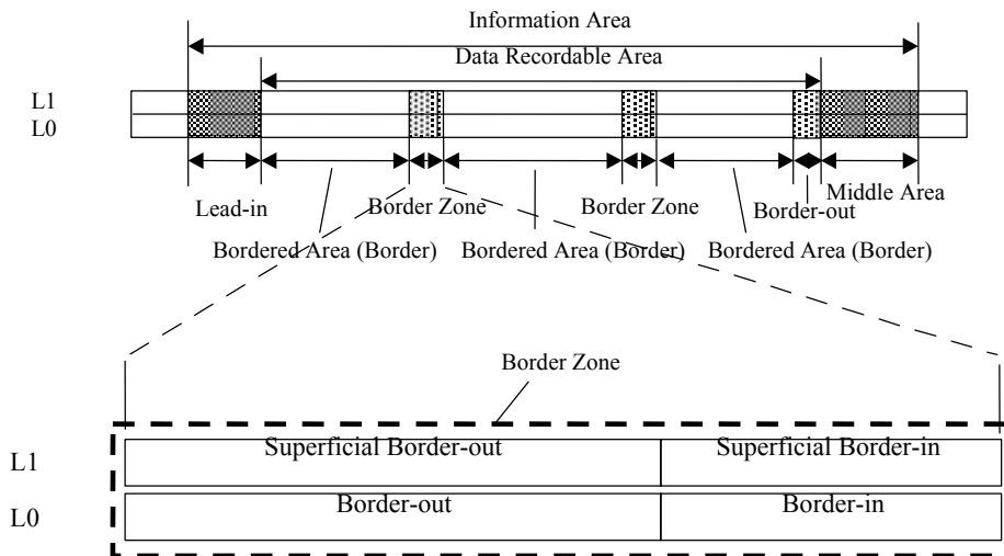
Figure 39 — Border Zone Structure for DVD-R Dual Layer media
