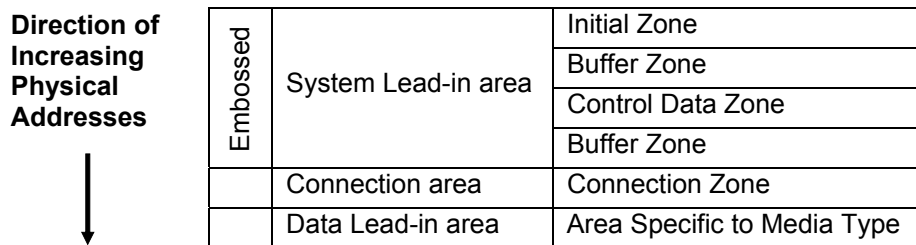
Figure 71 — General Layout of Lead-in area
