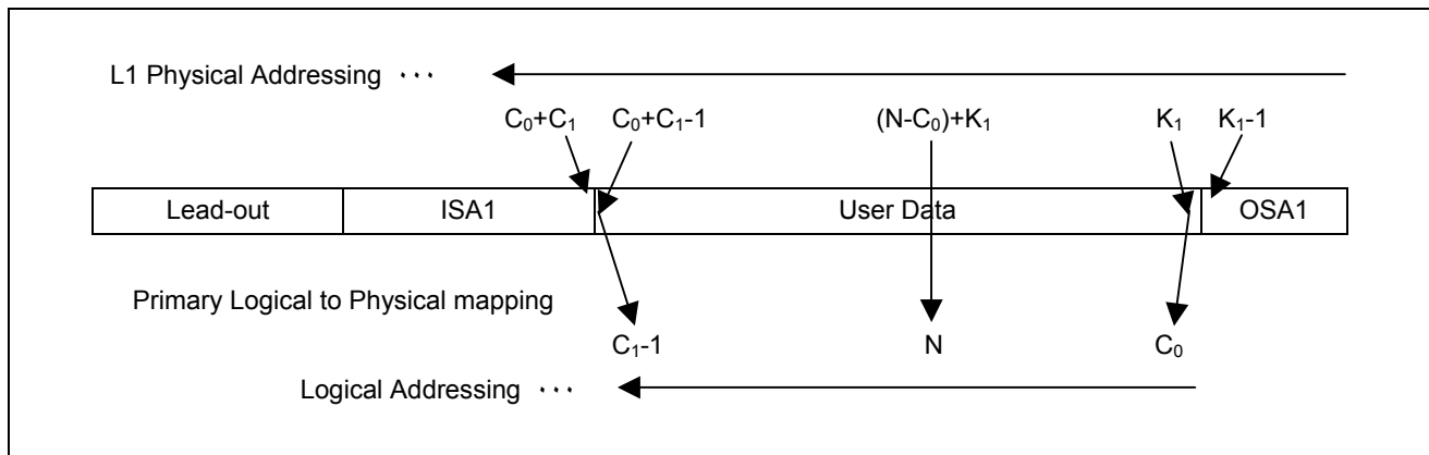
Figure 90 — Logical to Physical Addressing on Dual Layer
