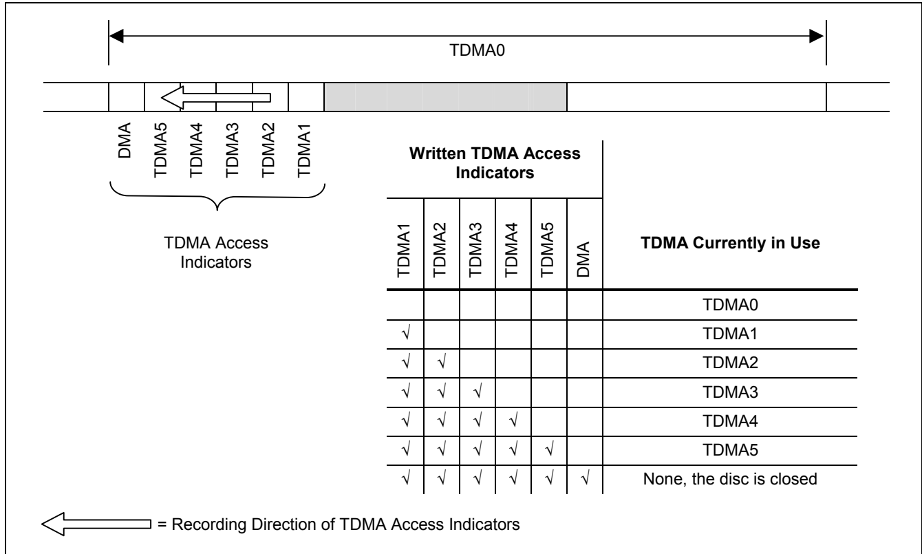
Figure 88 — TDMA Access Indicators on Dual Layer Disc
