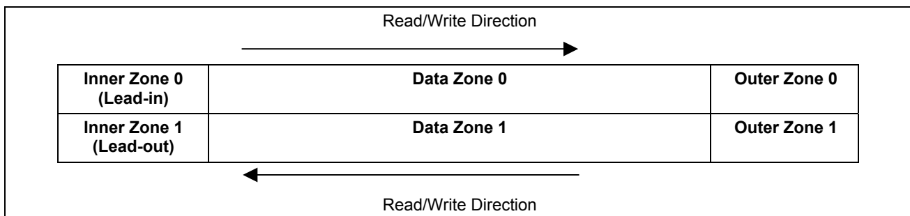
Figure 81 — Primary Zones of a Dual Layer BD-R
