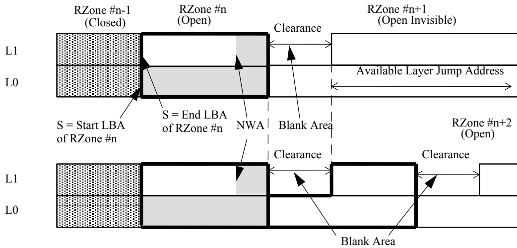
Figure 38 — Blank Areas and RZone Shape
