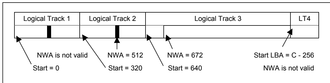
Figure 101 — Status after writing to Logical Track 1
