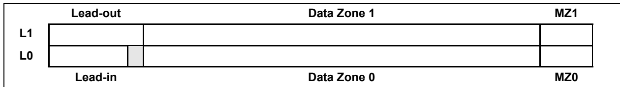
Figure 59 — Foreground part of the format process
