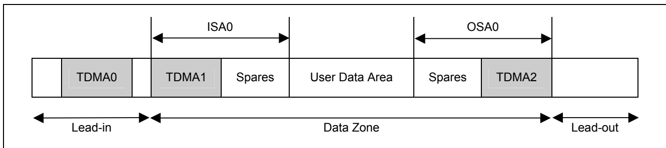
Figure 84 — TDMA Allocation on SL BD-R
