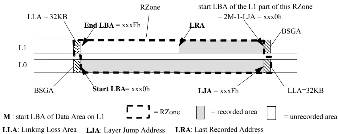
Figure 37 — RZone structure for Layer Jump recording
