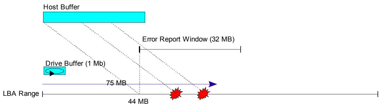
Figure 119 — Defects appear in the Error Report Window
