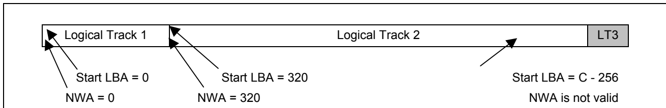
Figure 97 — Status after Splitting Logical Track 1
