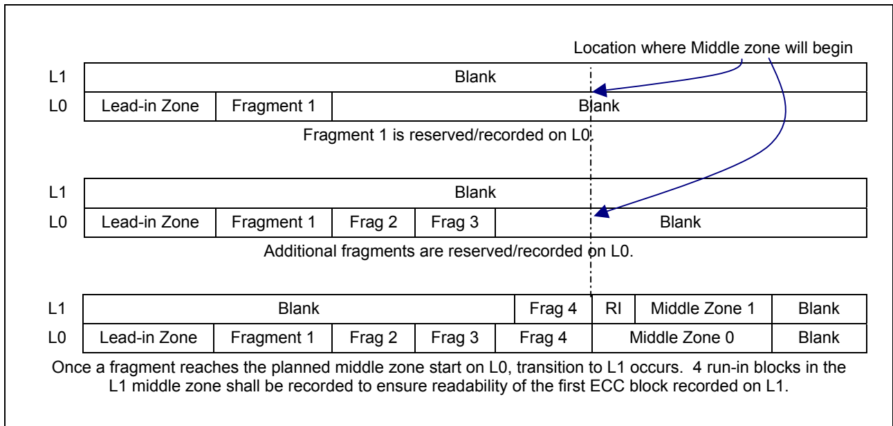
Figure 54 — Example: Crossing the Layers During Recording
