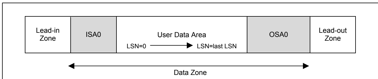
Figure 103 — Layout of Single Layer BD Disc
