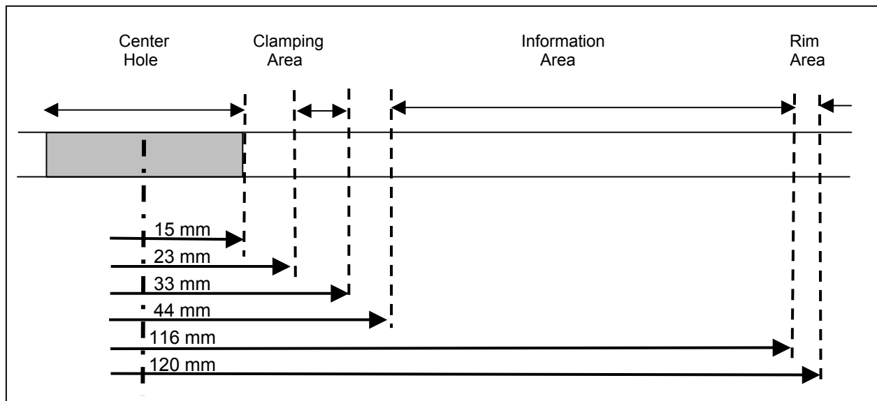
Figure 67 — The Areas of a HD DVD Medium
