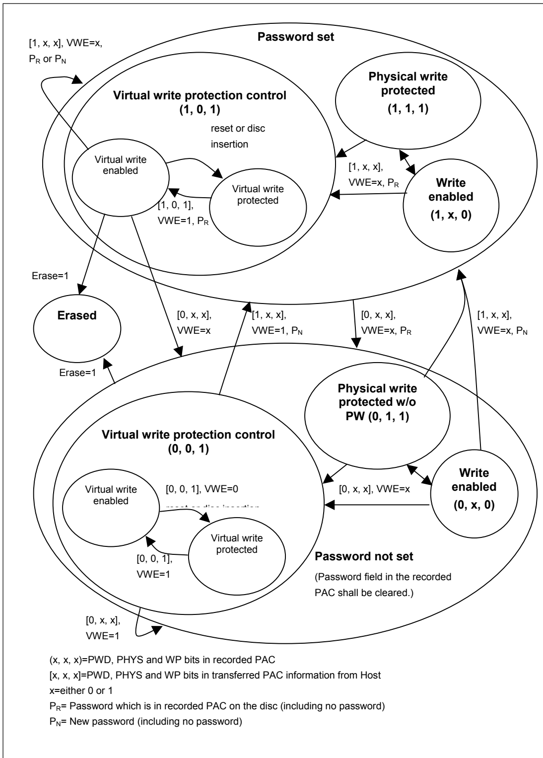
Figure 108 — Physical and Virtual Write Protect State Diagram
