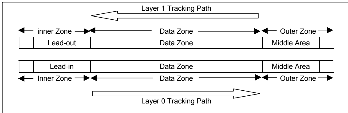
Figure 5 — General Dual Layer OTP Structure
