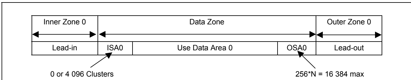
Figure 83 — SL BD-R Information Zone
