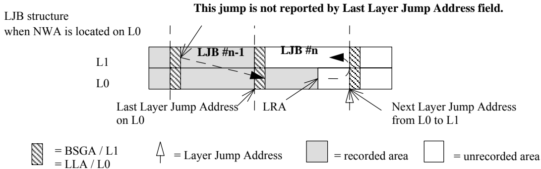
Figure 41 — LJB Structure of Invisible/Incomplete RZone
