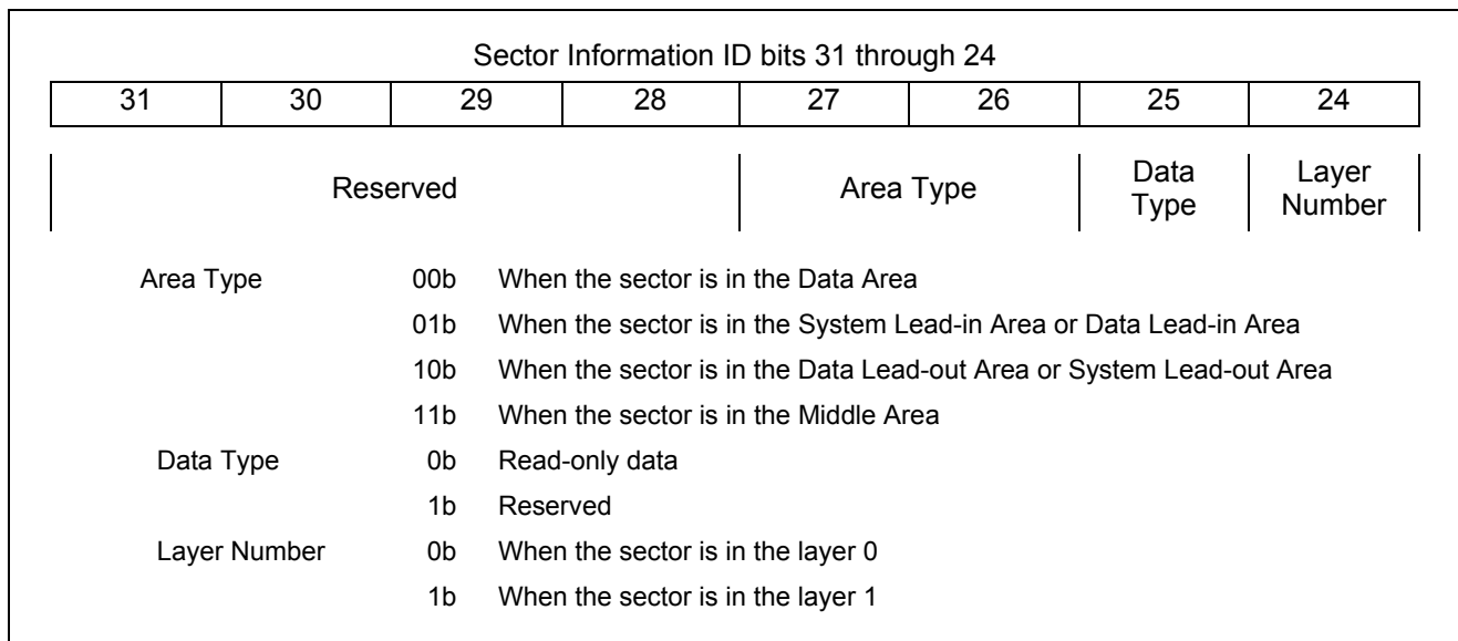
Figure 72 — HD DVD-ROM ID field Sector Information details
