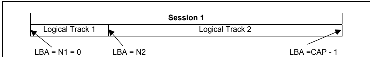
Figure 92 — Status of BD-R Disc After First RESERVE TRACK Command
