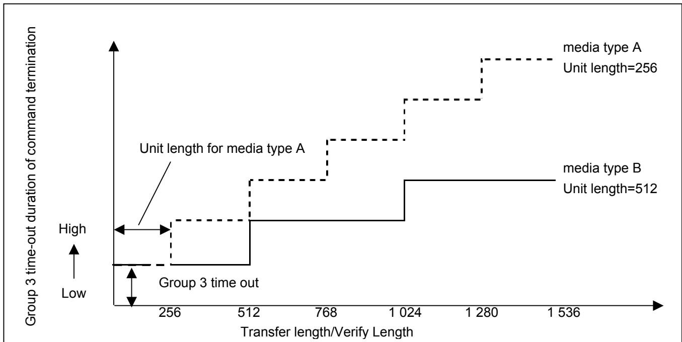
Figure 8 — Adjustment of Command Termination Time on Different Media
