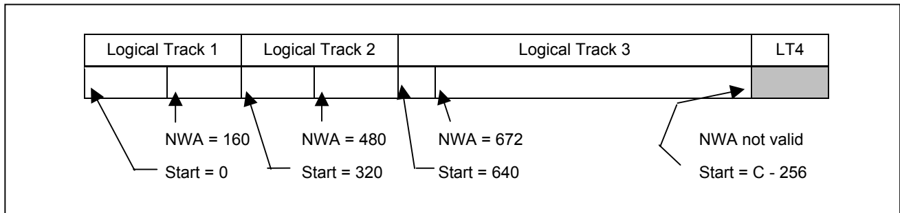
Figure 99 — Status after Writing to each Logical Track
