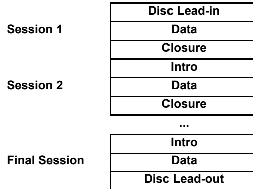
Figure 46 — General Layout of a Multi-Session DVD+R
