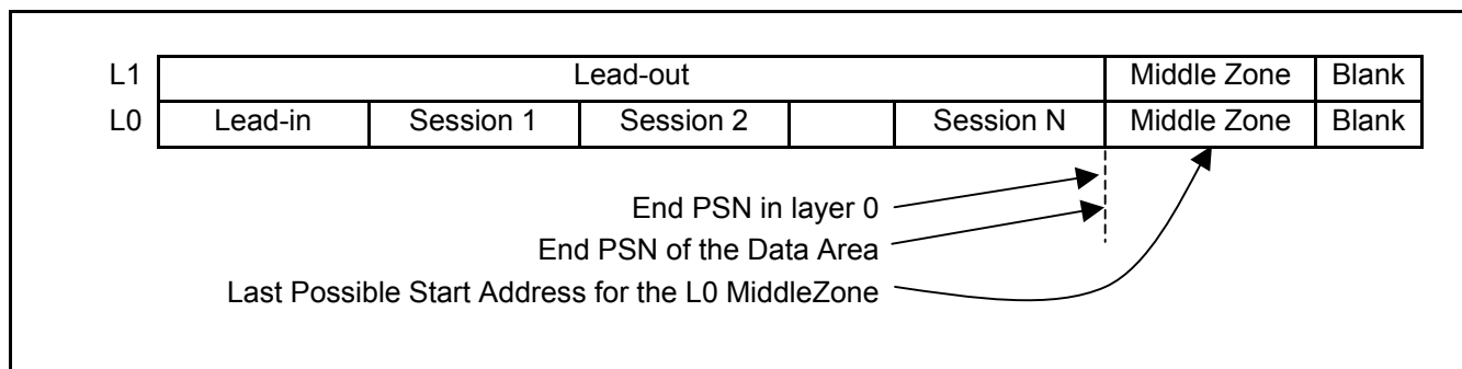
Figure 52 — Preferred Single Layer Recording
