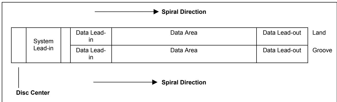
Figure 74 — Single Layer, Single Sided Disc
