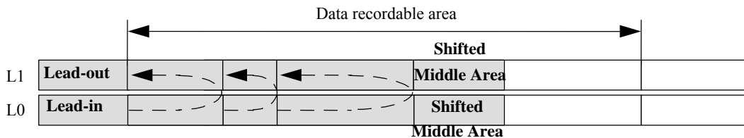
Figure 44 — Disc Final Closure in Layer Jump Recording Mode
