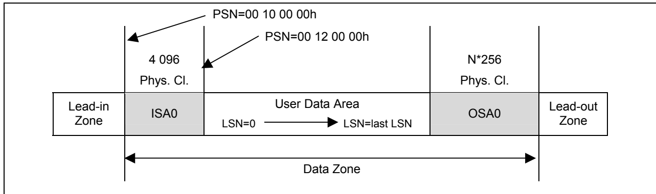
Figure 106 — Layout of Single Layer BD-RE Disc
