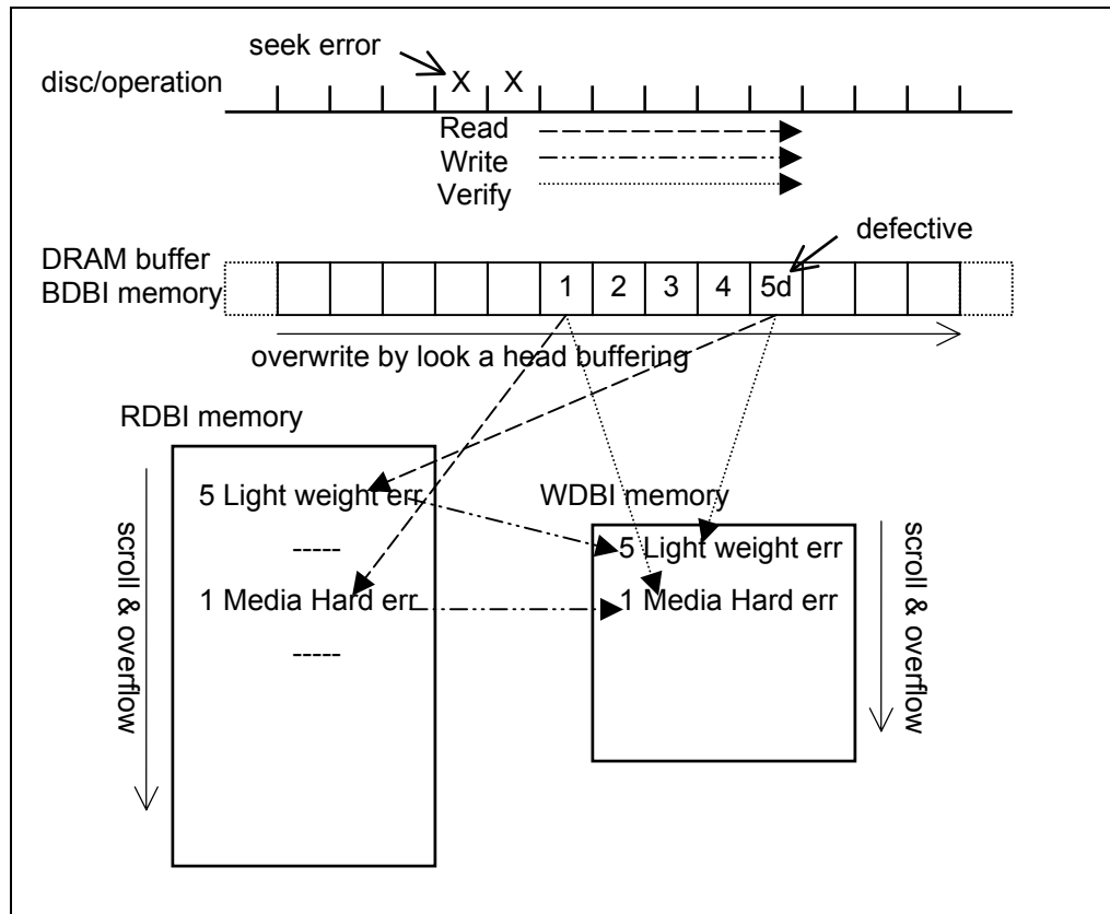
Figure 111 — Example of DBI memory blocks
