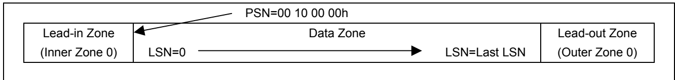
Figure 77 — Layout of Single Layer BD-ROM Information Zone
