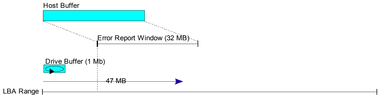
Figure 118 — Recording continues with no discovered defects
