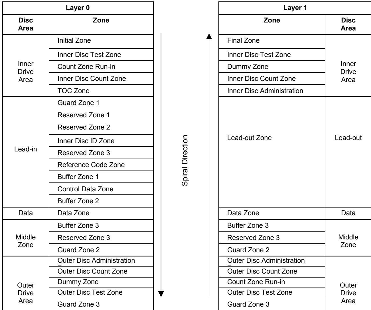
Figure 49 — Logical Layout of a DVD+R DL Disc
