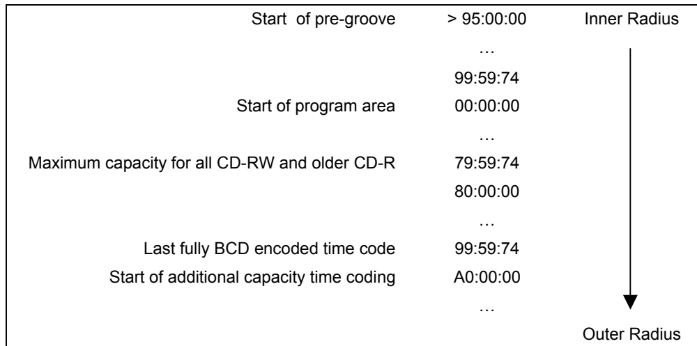
Figure 19 — Time Codes in CD-R and CD-RW Pre-groove
