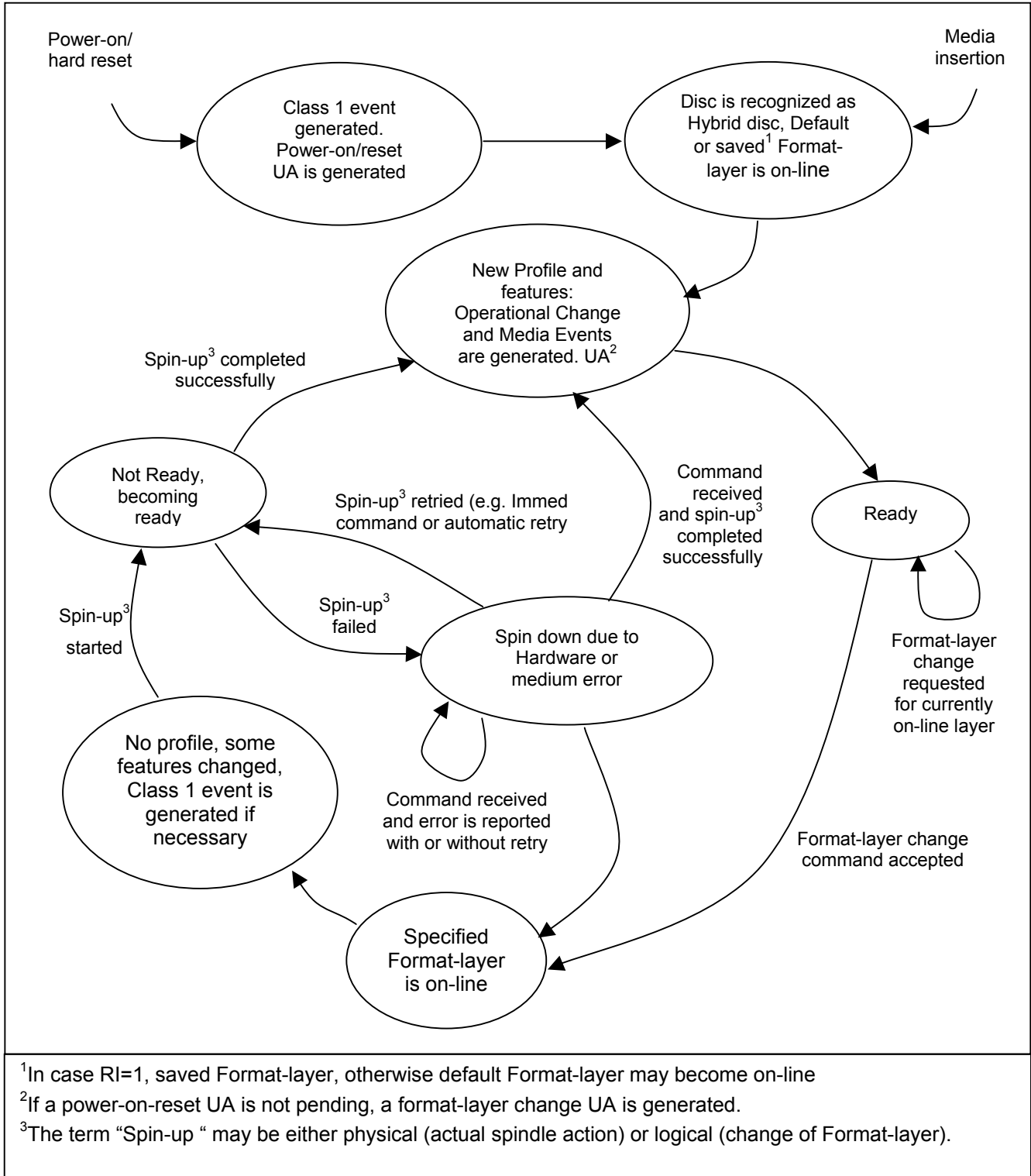
Figure 126 — State diagram of Format-layer changing
