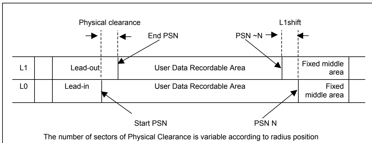
Figure 35 — Physical Overview of Layers
