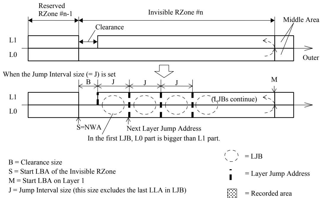
Figure 42 — Regular Interval Layer Jump
