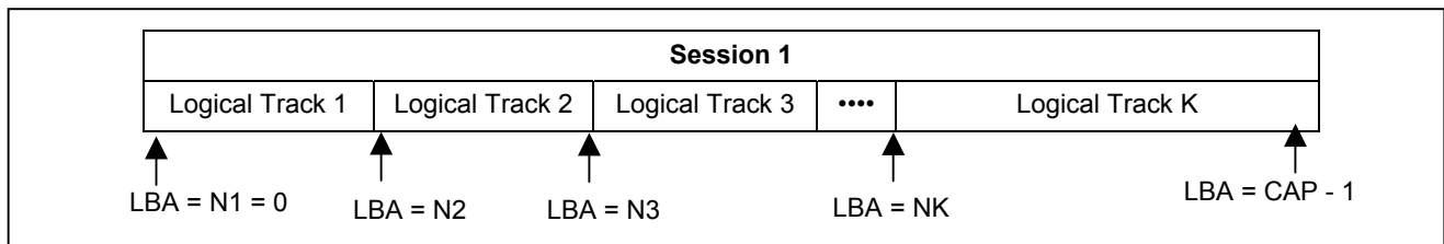
Figure 93 — Status of BD-R Disc Multiple RESERVE TRACK Commands
