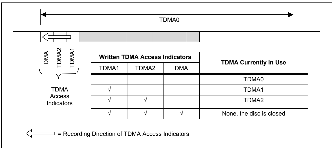
Figure 87 — TDMA Access Indicators on Single Layer Disc
