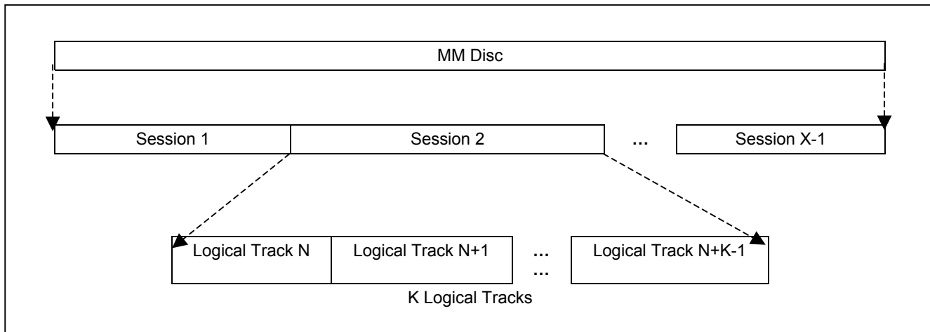
Figure 7 — Disc, Session and Logical Track Decomposition
