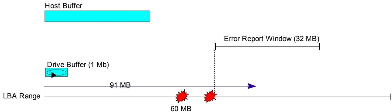
Figure 121 — Error Report Window Range is beyond known defects
