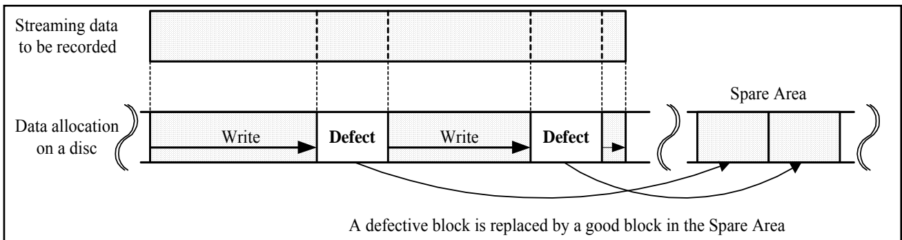
Figure 113 — Example of Data Allocation in case of Linear Replacement
