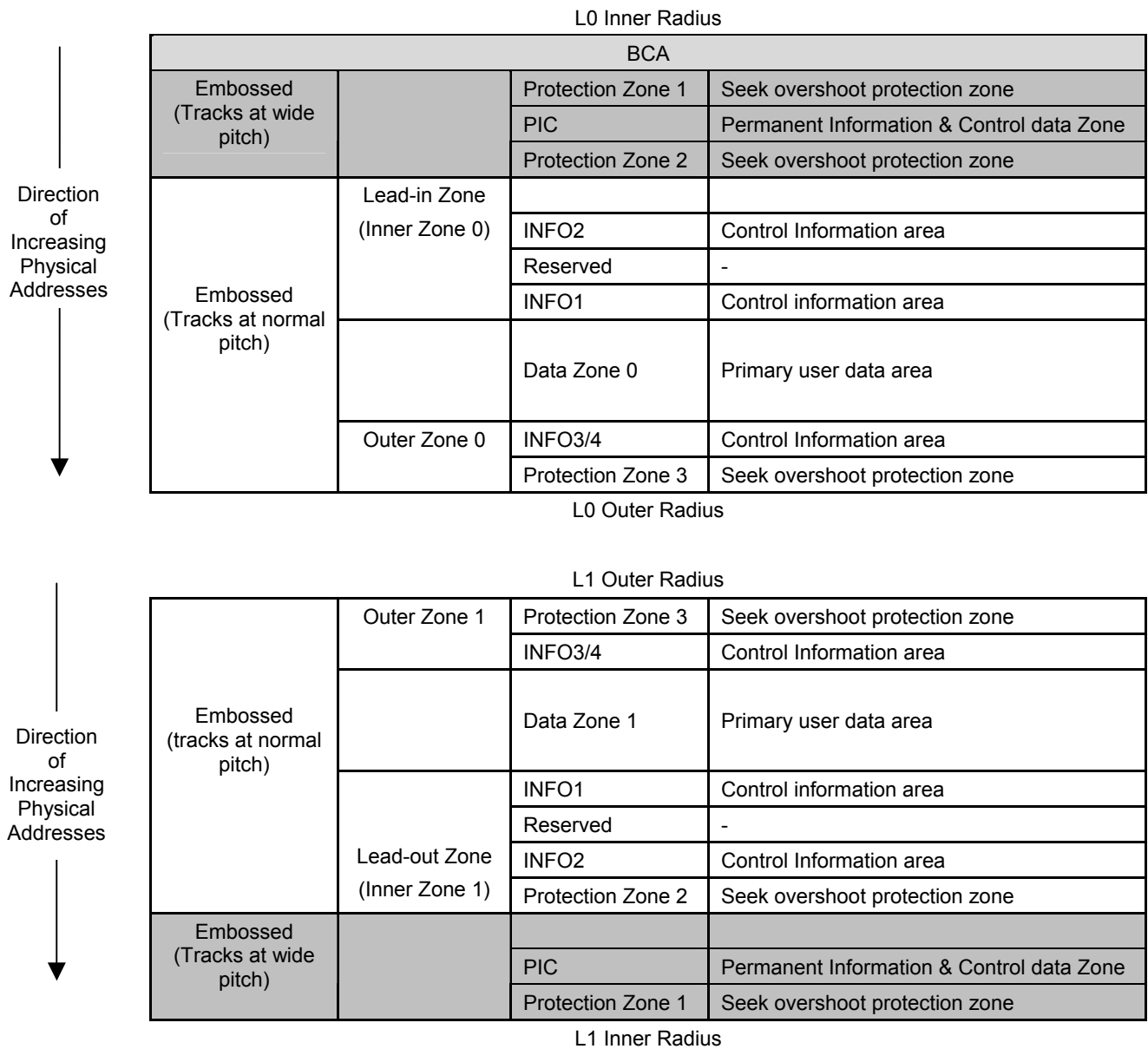
Figure 79 — BD-ROM Information Zone
