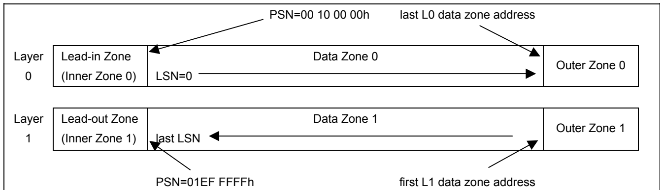
Figure 78 — Layout of Dual Layer BD-ROM Information Zone
