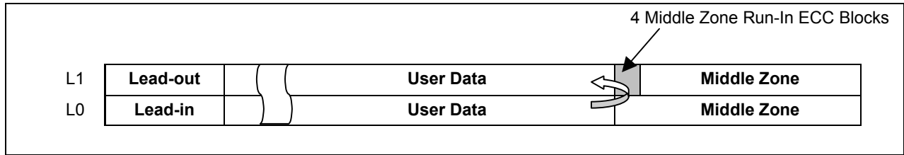
Figure 53 — Run-in ECC Blocks in L1 Middle Zone
