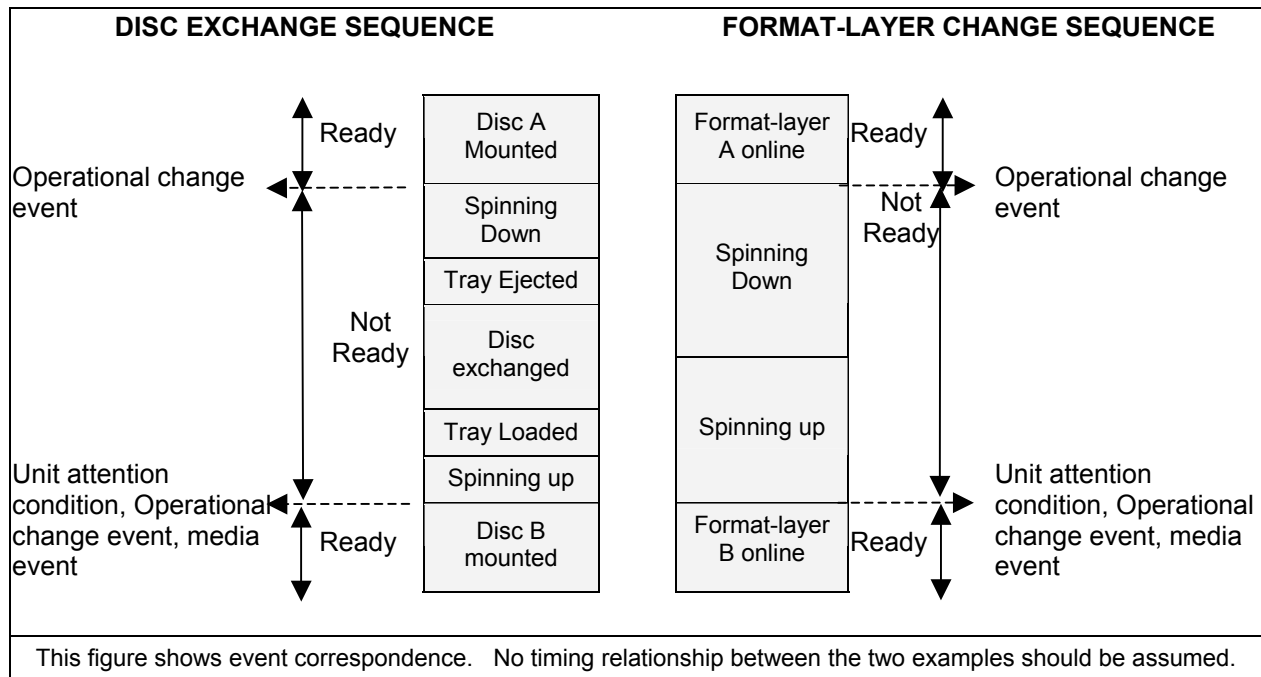
Figure 125 — Comparison of disc exchange and Format-layer change
