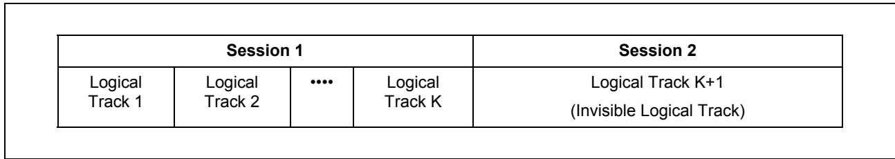
Figure 94 — Status of BD-R Disc after Closing Session 1
