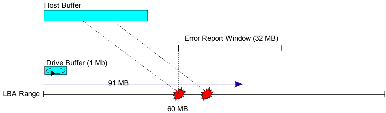
Figure 120 — Last Chance to Notify Host of Defects
