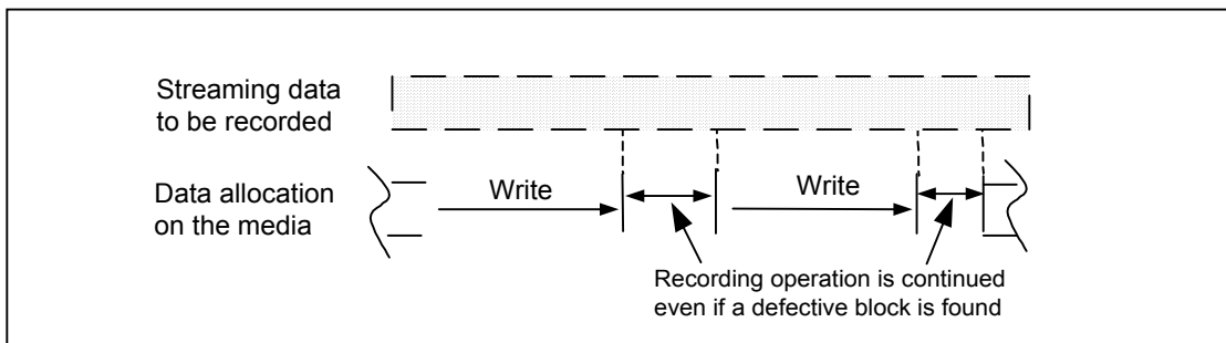
Figure 114 — An example of data allocation on the Stream recording operation
