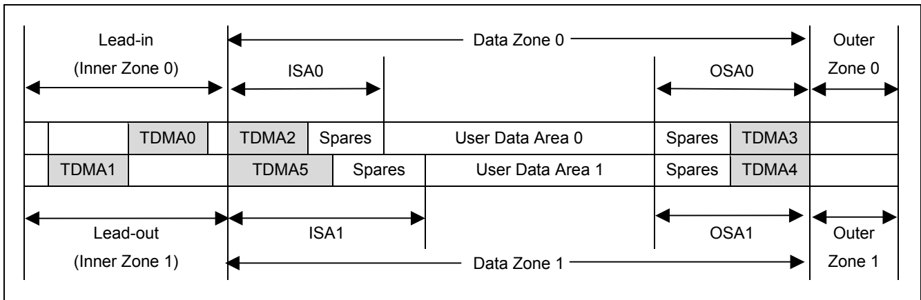
Figure 86 — TDMA Allocation on DL BD-R
