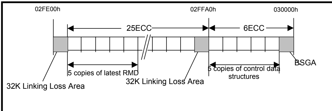
Figure 33 — Structure of Extra Border Zone
