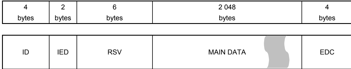
Figure 24 — Logical Layout of a DVD Data Sector
