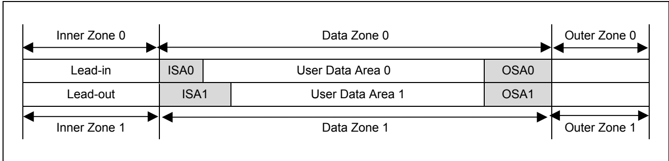
Figure 85 — DL BD-R Information Zones
