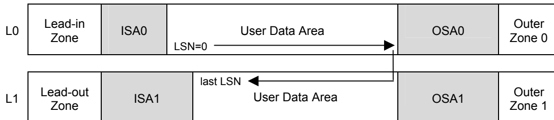
Figure 104 — Layout of Dual Layer BD-RE Disc
