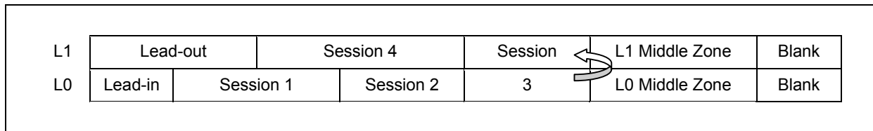
Figure 51 — Example of a DVD+R DL Disc
