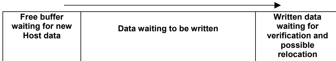
Figure 115 — Buffered Data Status
