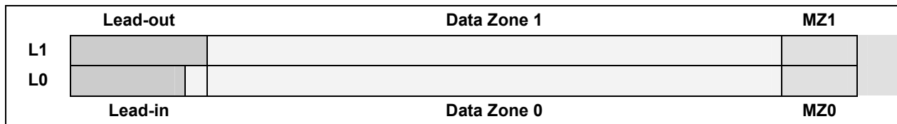
Figure 66 — Finalization part of the format process
