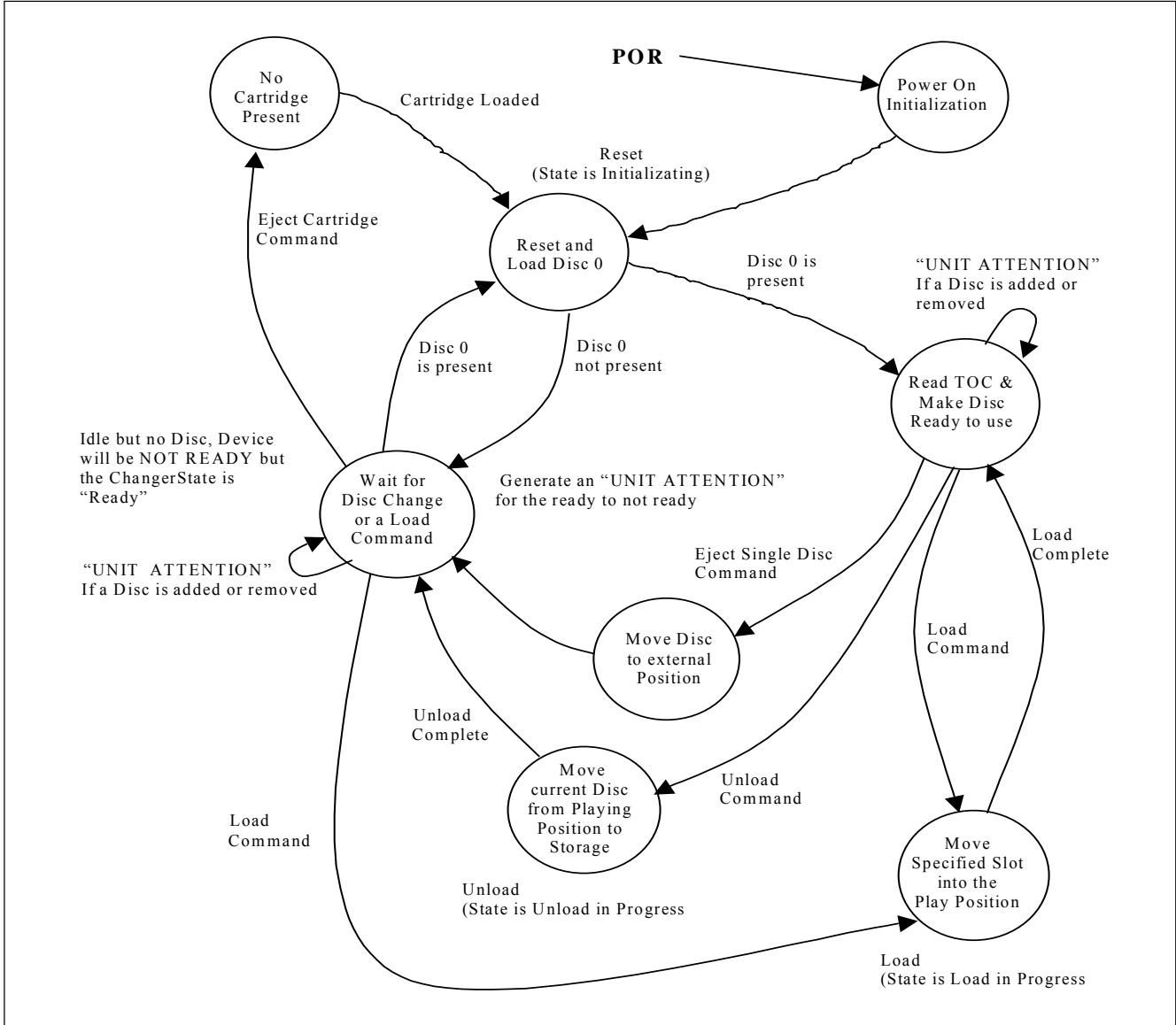
Figure 123 — Changer State Diagram
