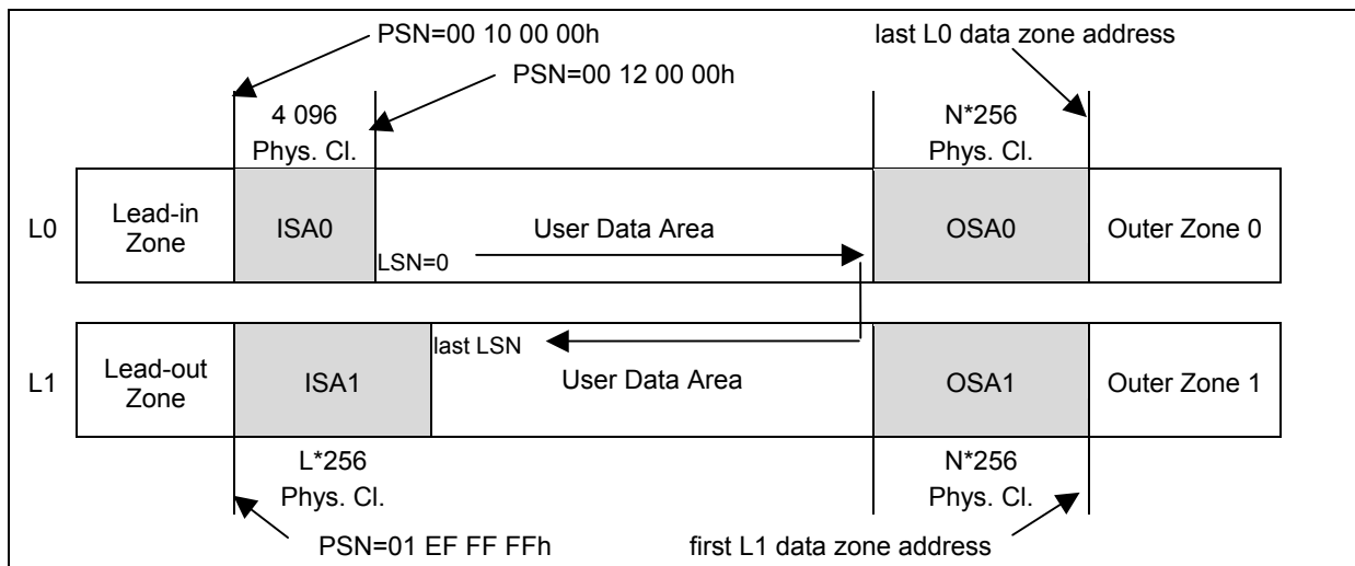
Figure 107 — Layout of Dual Layer BD-RE Disc
