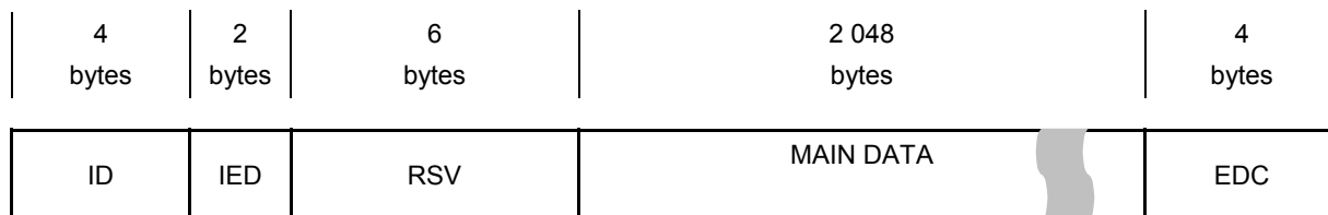
Figure 68 — Logical Layout of a HD DVD Data Sector
