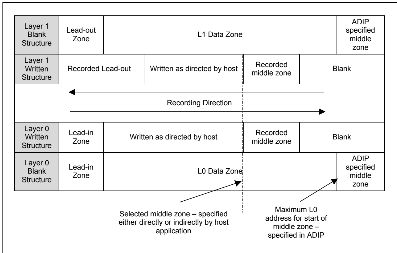
Figure 50 — Blank and Recorded Structure of a DVD+R DL Disc
