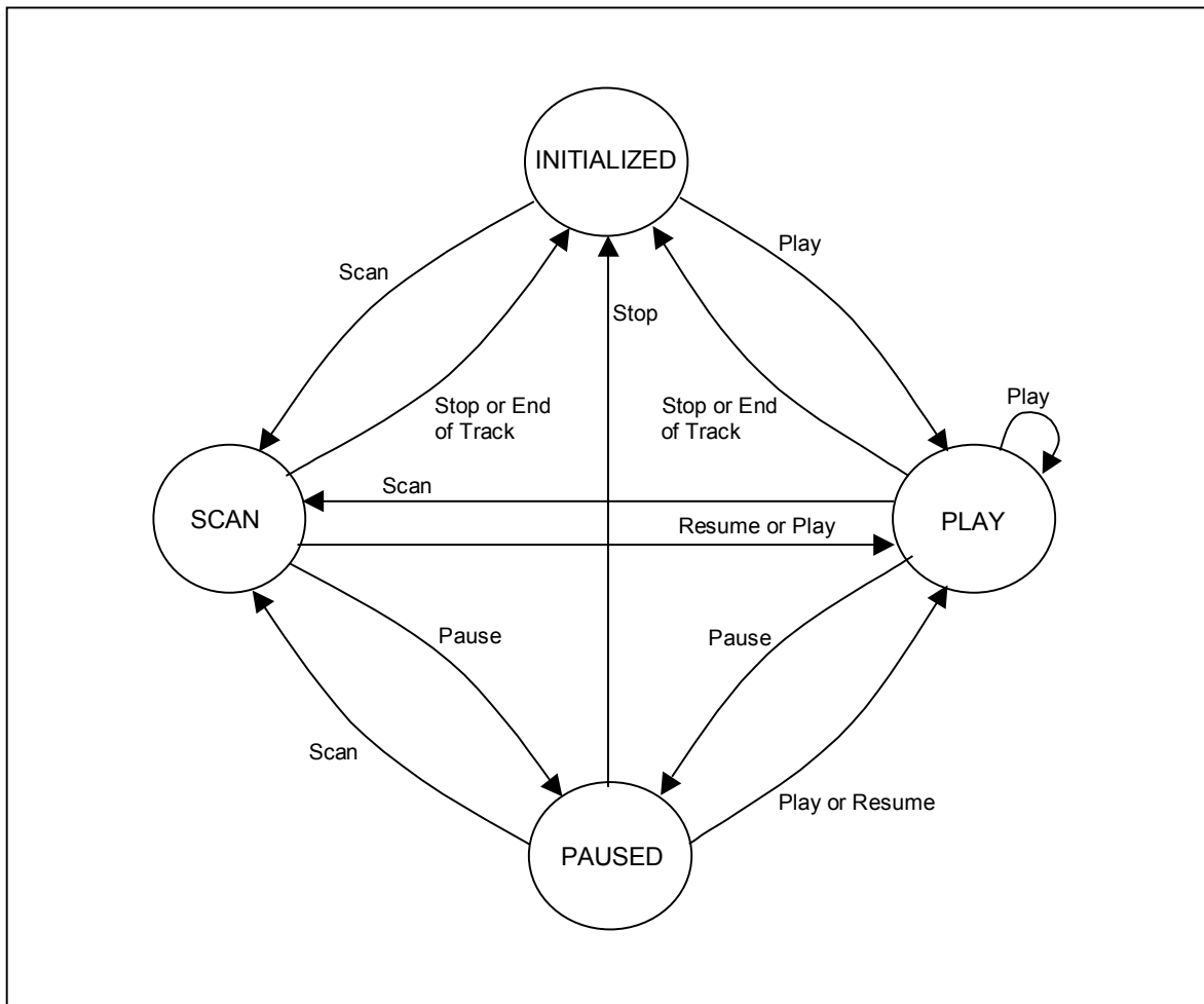
Figure 50 – Stop Play/Play Audio/Audio Scan/Pause/Resume Sequencing
