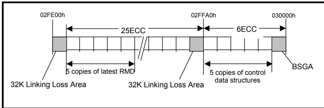
Figure 35 – Structure of Extra Border Zone
