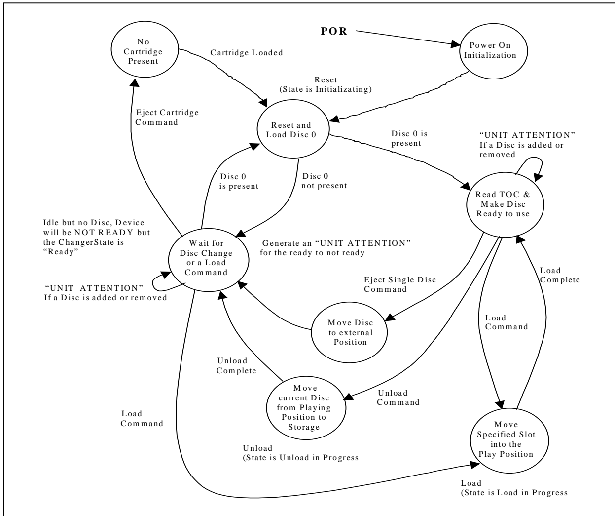
Figure 46 – Changer State Diagram
