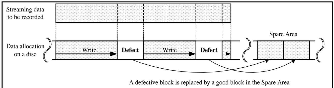
Figure 43 – Example of Data Allocation in case of Linear Replacement
