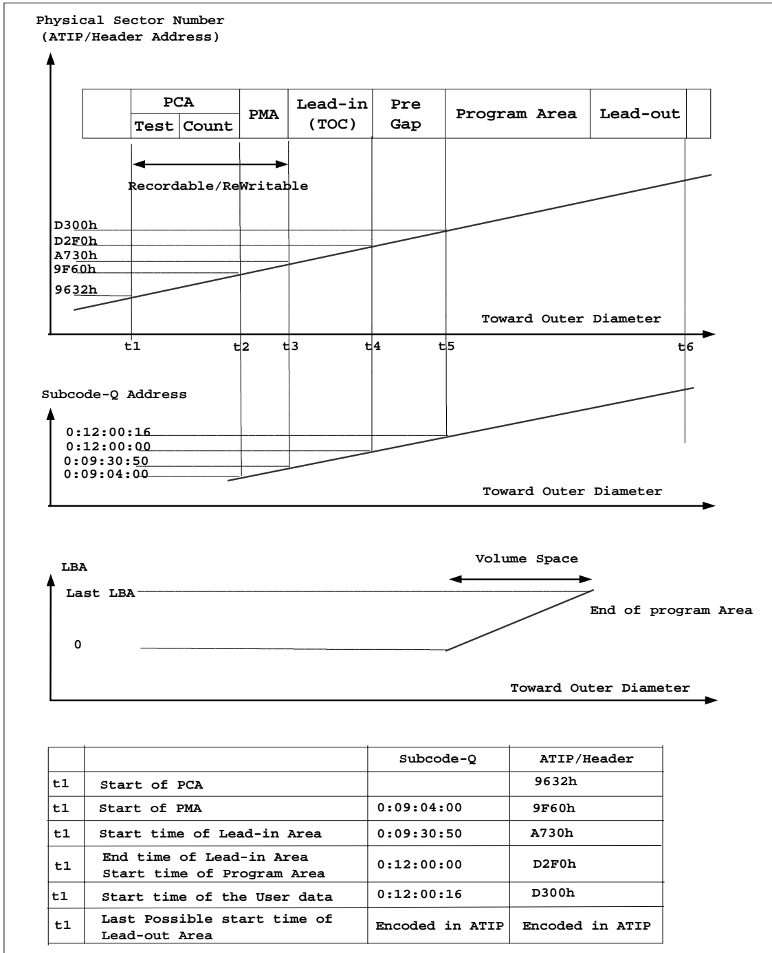
Figure 18 – Physical and Logical Layout of DDCD-ROM/R/RW
