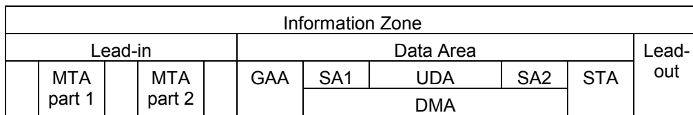
Figure J.3 – MRW Mapping onto DVD+RW, General
