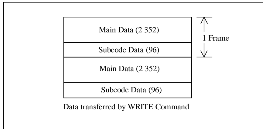
Figure 49 – Location of Sub-channel Data
