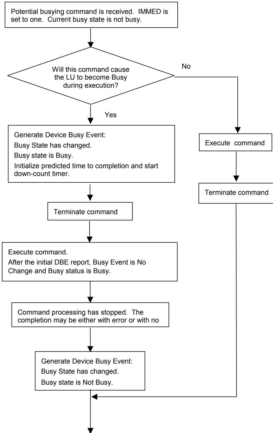
Figure 48 – Execution of a command that may cause Logical Unit Busy
