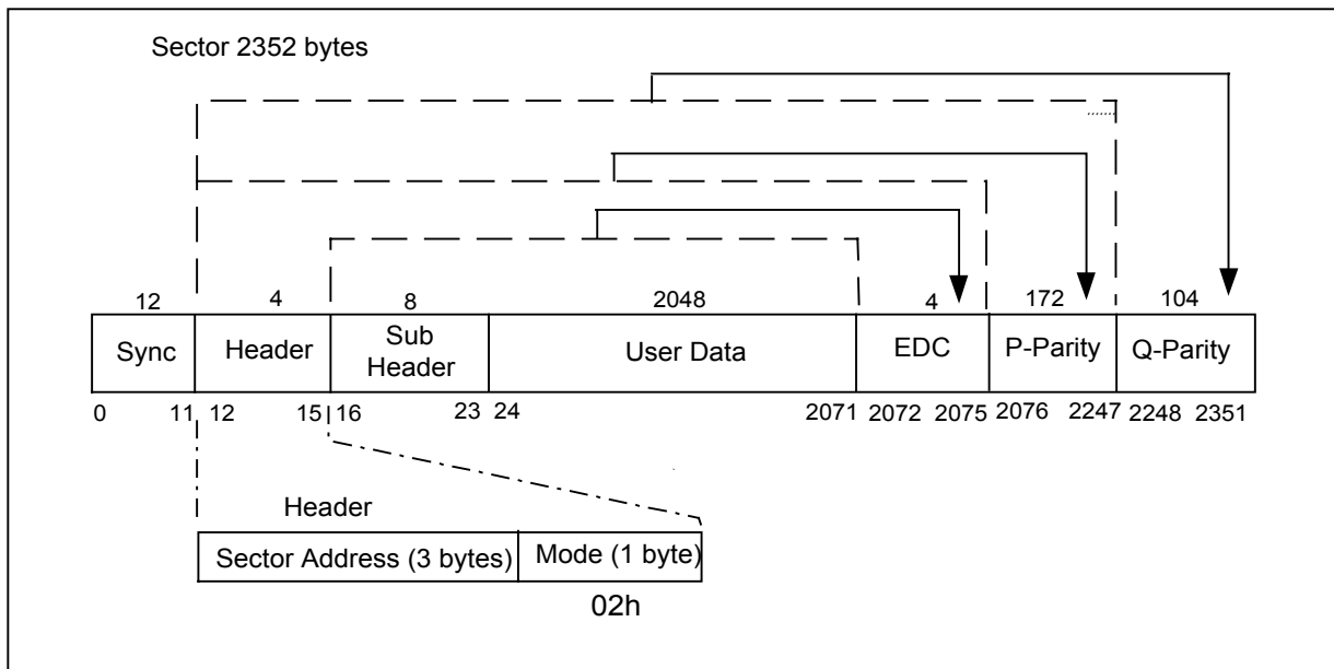
Figure 20 – Sector format Mode 2
