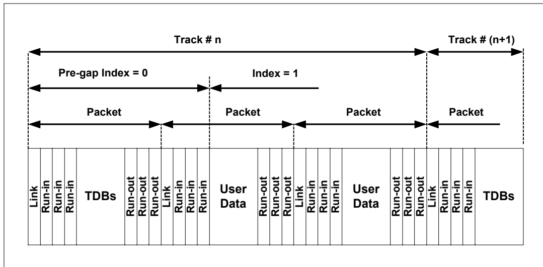
Figure 23 – Example of Packet written Track layout
