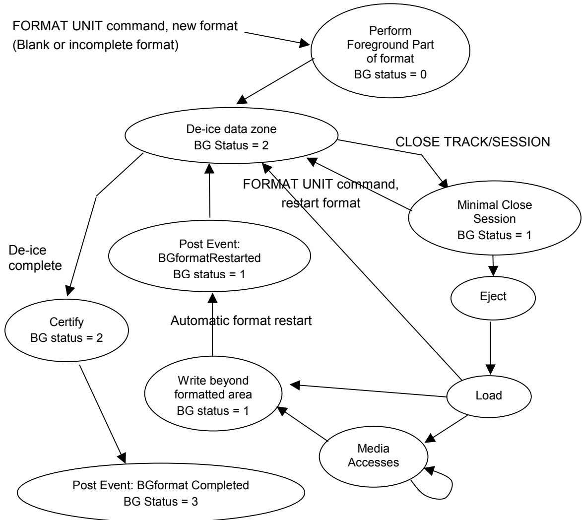
Figure 47 – Background Process Flow
