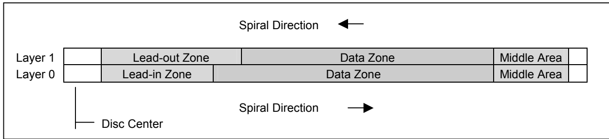
Figure 27 – Opposite Track Path Disc
