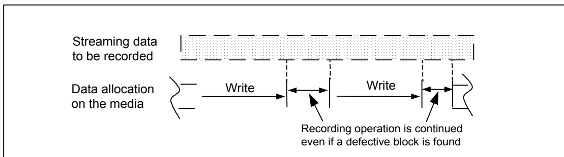
Figure 44 – An example of data allocation on the Stream recording operation
